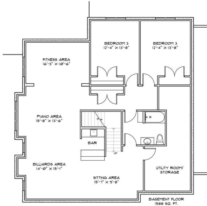
BASEMENT FLOOR PLAN SCALE 3/32" = 1'-0"
